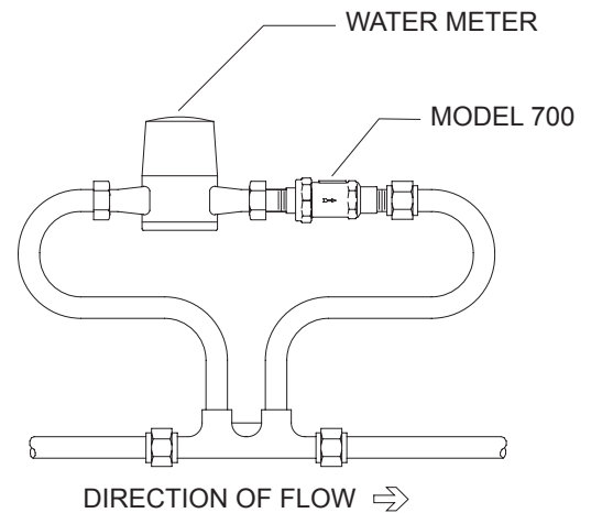
METER SETTER INSTALLATION
