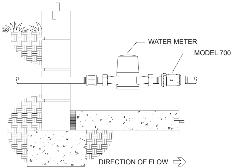
INDOOR INSTALLATION
