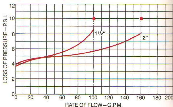
Head Loss — 1 1/2" and 2"
