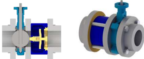
Shown with Flomatic® Model 888S6VFD wafer check valve close coupled with Sylox®3 butterfly valve. Butterfly valve can be operated with check valve in an “open” or “closed” position with no interference.
