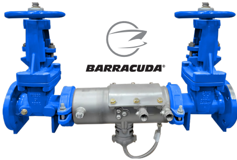
FRP2.50-SS-OSY-BA (ILLUSTRATED) FOR SPEC. SHEETS GO TO www.beecobackflow.com
