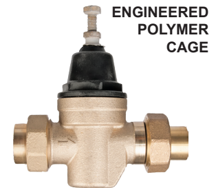
PRV.75-DU-IPS-C-LL (ILLUSTRATED)
