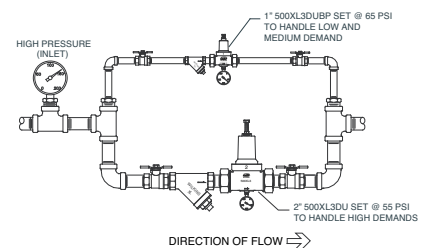
PARALLEL INSTALLATION
