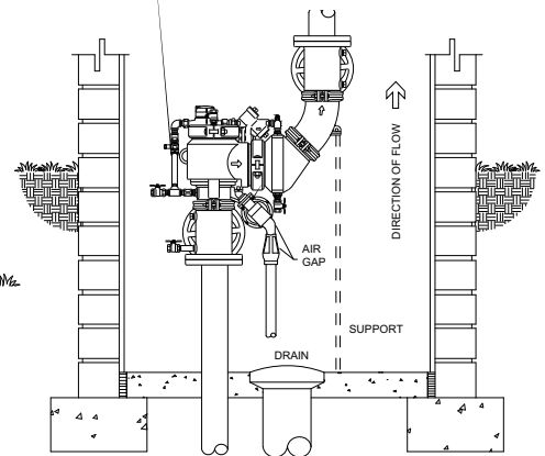
VERTICAL INSTALLATION (MODEL 475DAV)
