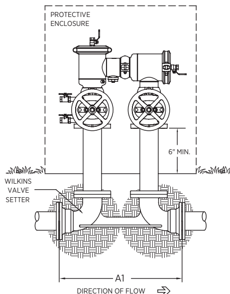
OUTDOOR INSTALLATION
