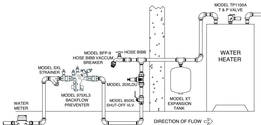
OUTDOOR INSTALLATION
