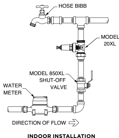
INDOOR INSTALLATION
