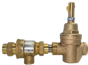
BCOMBO.75-NPT (ILLUSTRATED)
