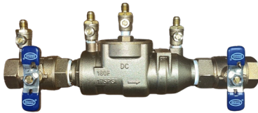
FDC.75-QT-LL (ILLUSTRATED)
